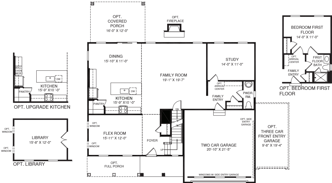
MAIN LEVEL
