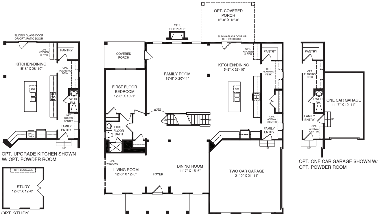
MAIN LEVEL
