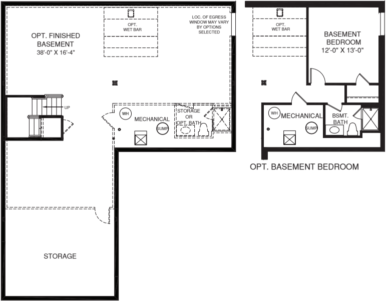
LOWER LEVEL
