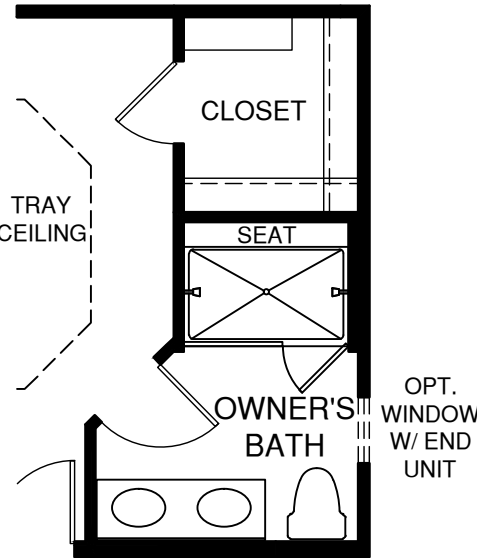
OPT. OWNER'S BATH SHOWER ALT. LAYOUT
