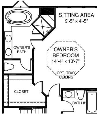
OPT. OWNER'S BATH W/ 6' EXT.
