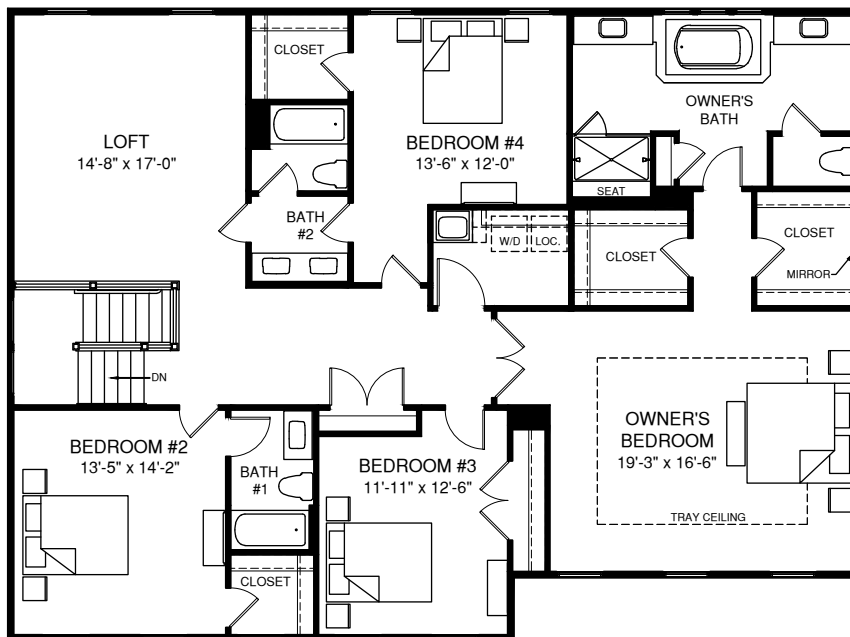
FOUR BEDROOM W/ OPT. LOFT
