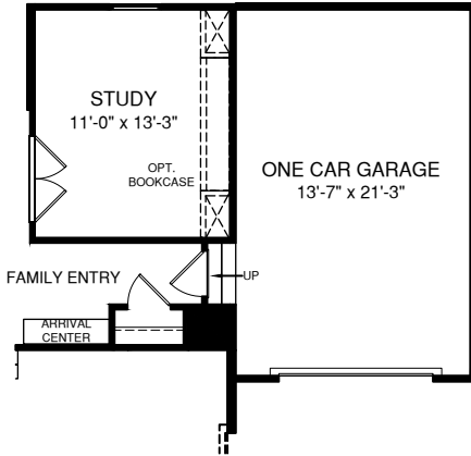
OPT. ONE CAR GARAGE ONLY AVAILABLE W/ OPT. SIDE ENTRY GARAGE
