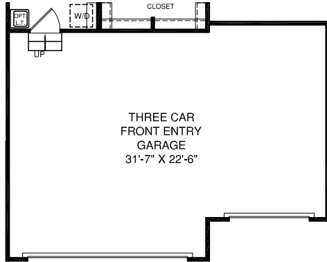
OPT. THREE CAR FRONT ENTRY GARAGE
