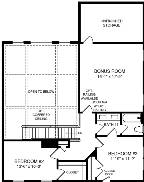
OPT. THREE BEDROOM W/ BONUS ROOM
