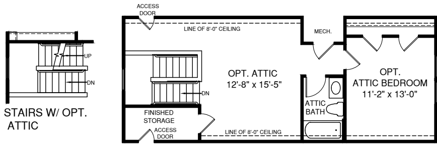
OPT. ATTIC W/ OPT. ATTIC BEDROOM
