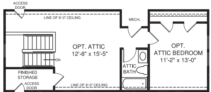
OPT. ATTIC W/ OPT. ATTIC BEDROOM
