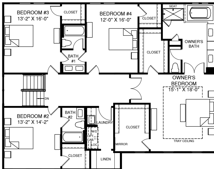
OPT. OWNER'S BATHROOM W/ FREESTANDING TUB
